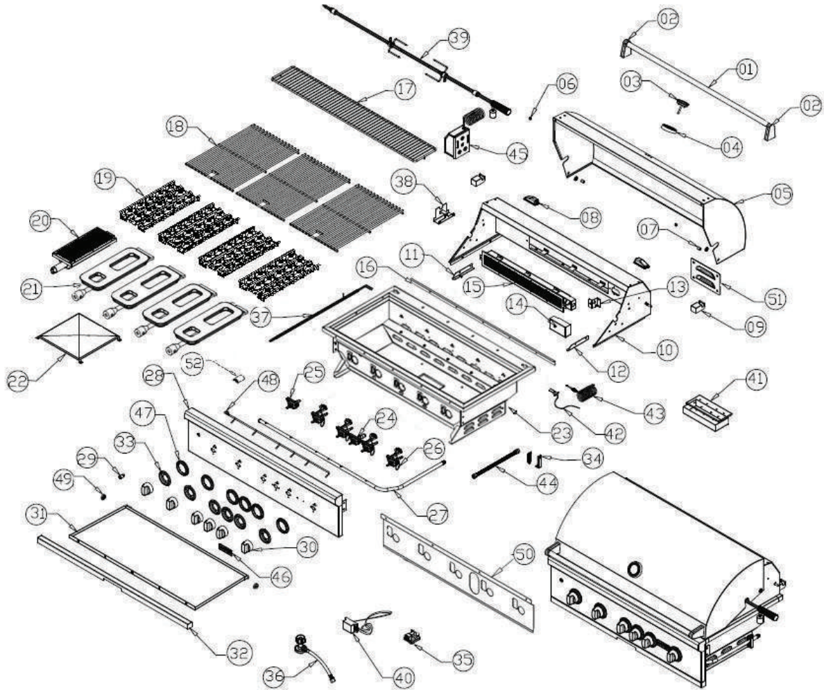
C2SL42 Parts Listing
